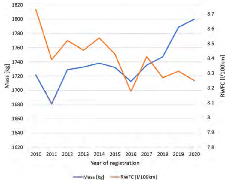
Figure 3-3: Trend of average vehicle mass and real-world fuel consumption per registration year for diesel vans (excl. plug-in hybrids).
