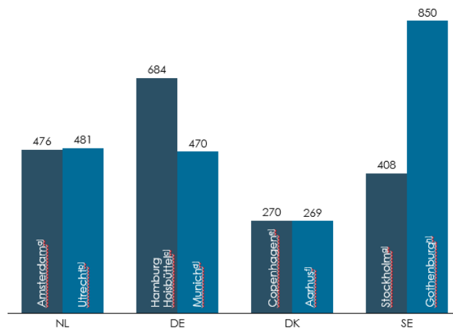
Figure 1 Fixed tariff shares of district heating tariffs EUR/year/10kW connection capacity
