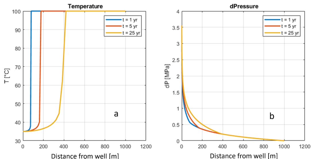
Figure 6 Temperatures (a) and pressure changes (b) in the aquifer. Different colours indicated different times during injection.
