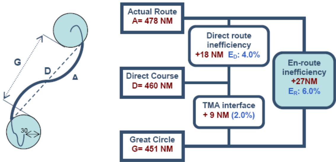
Figure 7: Illustration of flight efficiency indicators. Source: Eurocontrol Performance Review Commission 70 .
